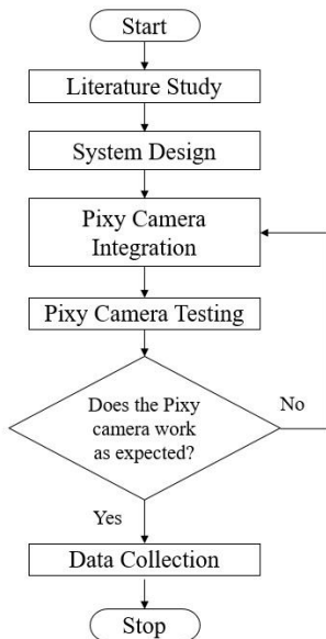
Fig. 1. Research Flowchart
